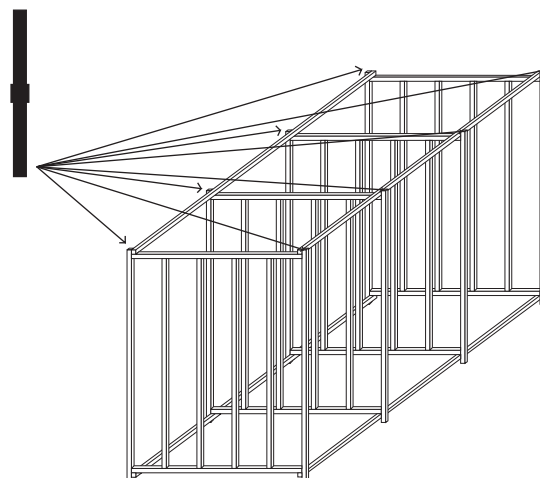
View of Double Stacked Storage Racks
